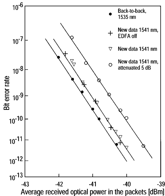
Fig. 5. BER measurements: (●) the original 2.5-Gb/s NRZ data at 1535 nm; (+) new 2.5-Gb/s NRZ data at 1541 nm with EDFA in the wavelength converter turned off; (▽) new 2.5-Gb/s NRZ data with the wavelength converter turned on; and (○) new 2.5-Gb/s NRZ data attenuated 5 dB, otherwise as ▽.
